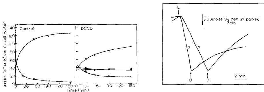
Fig. 5. The effect of 10^{-4} M ( \square , \square ) and 5 \cdot 10^{-4} M DCCD ( \bullet , \bullet ) on the net \text{Na}^+ extrusion ( \square , \bullet ) and \text{K}^+ influx ( \square , \bullet ). The suspensions were pretreated with DCCD for about 20 h at 5^\circ in the darkness. The figure also shows the control fluxes for \text{Na}^+ ( \square ) and \text{K}^+ ( \square ) obtained from cells treated in a similar way but without DCCD present. Other conditions were the same as for Fig. 4.
