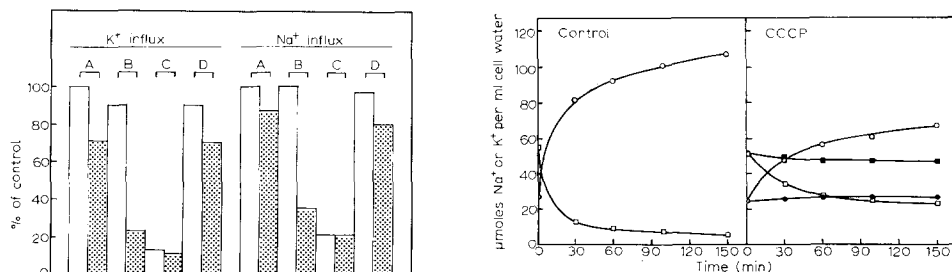
Fig. 3. The effect of various treatments on the initial rates of \text{Na}^+ - \text{K}^+ exchange induced from \text{Na}^+ -rich cells by adding 3 mM KCl. The cells were suspended in the \text{K}^+ -free medium given in the legend of Fig. 1 and were either illuminated (unshaded) or dark treated (shaded). The results are presented as the percentage of the light control. The various treatments were: (A) light and dark controls; (B) the magnitude of the light and dark fluxes measured under \text{N}_2 . The suspensions were pretreated with \text{N}_2 by bubbling for 1 h before injecting the \text{K}^+ ; (C) the net flux rates of \text{Na}^+ and \text{K}^+ at 1^\circ . The cells were pretreated for 30 min at this temperature before adding \text{K}^+ ; (D) the effect of 5 \cdot 10^{-5} M DCMU on the light and dark \text{Na}^+ - \text{K}^+ exchanges. Pretreatment time of 1 h.
